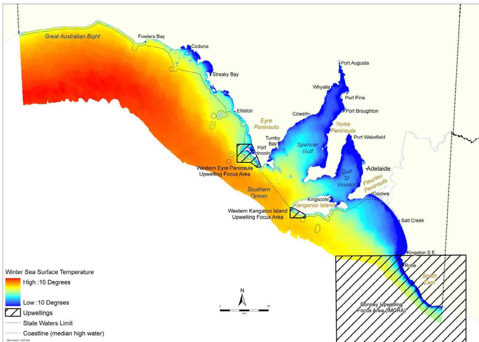
Figure 10: Winter sea surface temperature and upwelling areas
