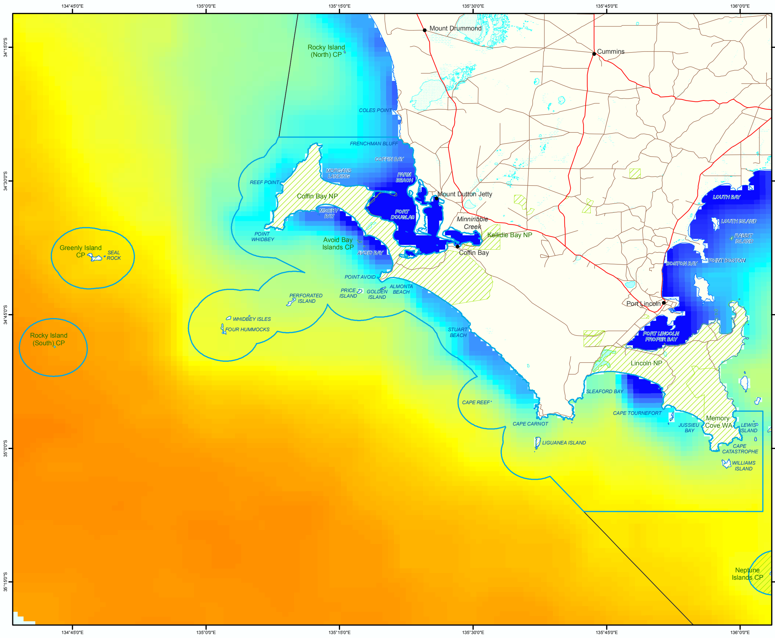
Figure 11: Thorny Passage Marine Park Average Winter Sea Surface Temperature
