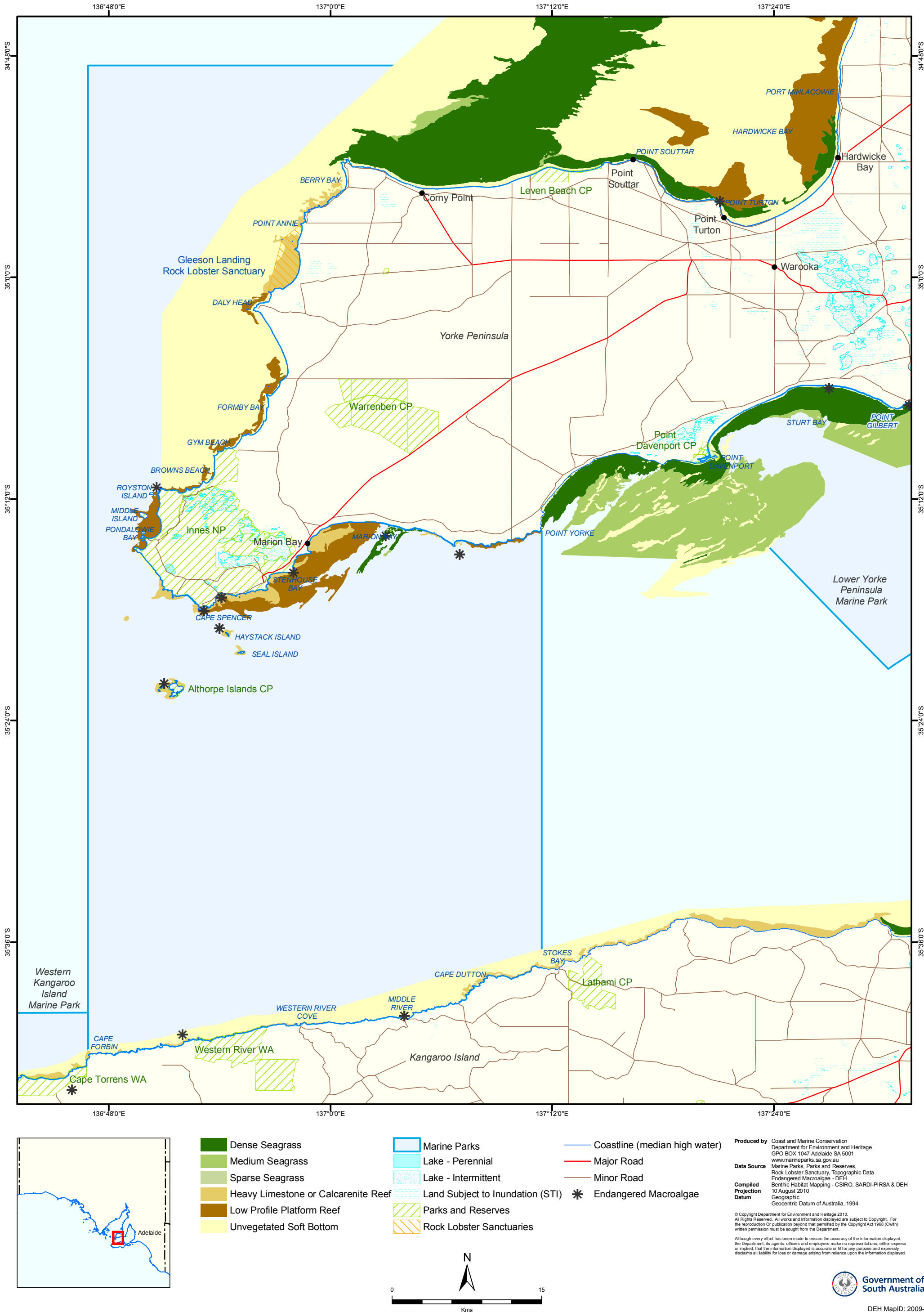
Figure 5A: Southern Spencer Gulf Marine Park National Benthic Habitats and Endangered Macroalgae
