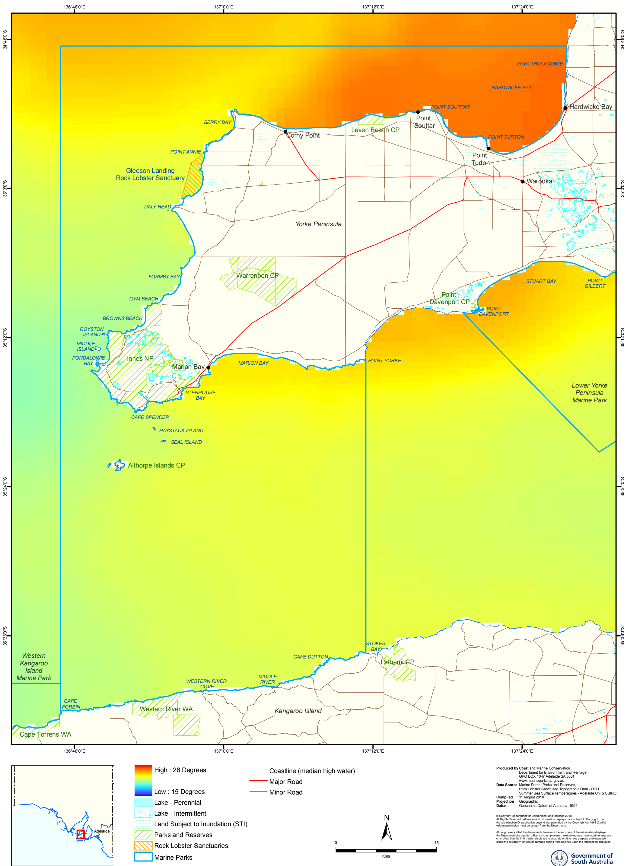
Figure 10: Southern Spencer Gulf Marine Park Average Summer Sea Surface Temperature
