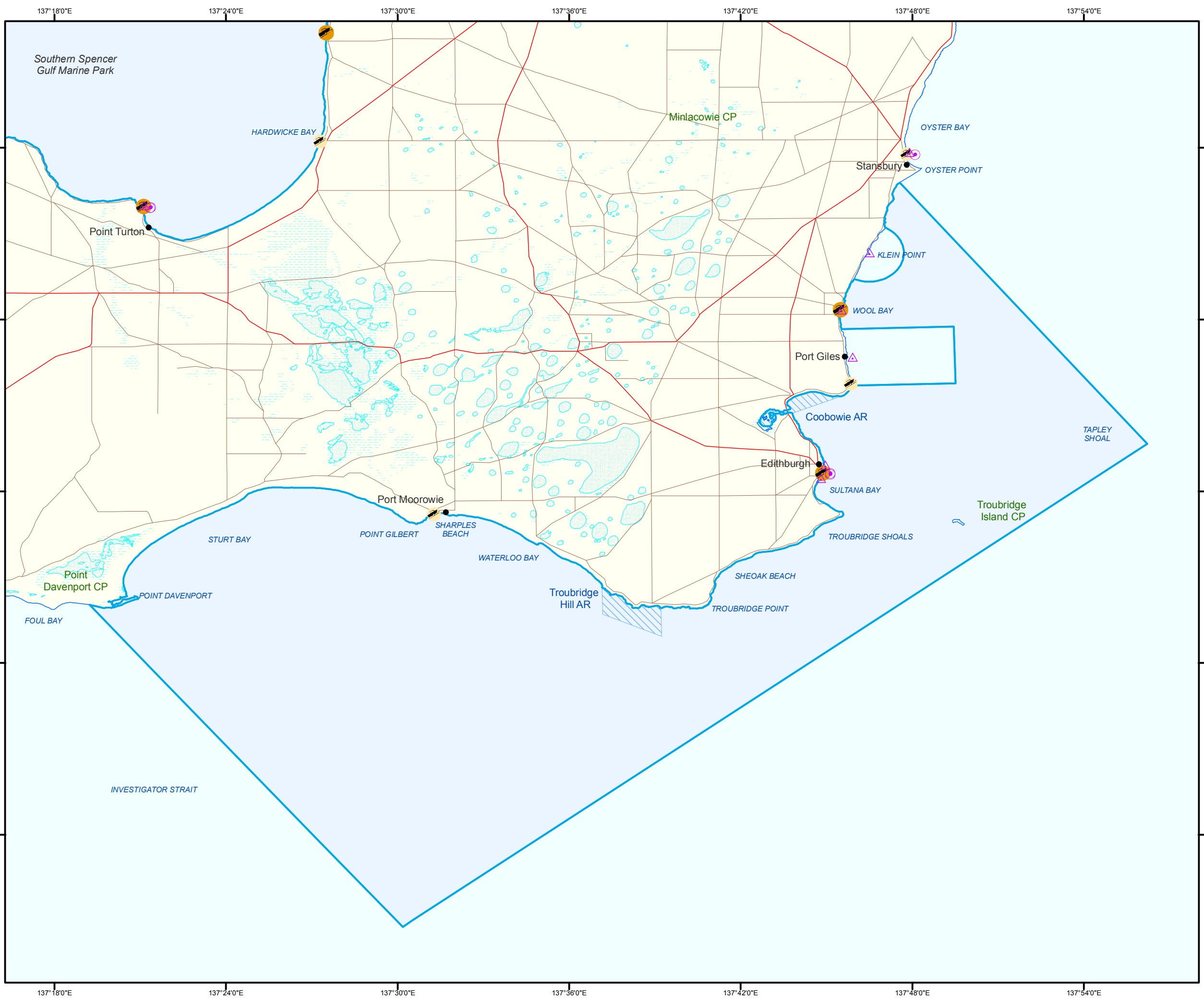
Figure 13: Lower Yorke Peninsula Boat Ramps, Breakwaters and Jetties
