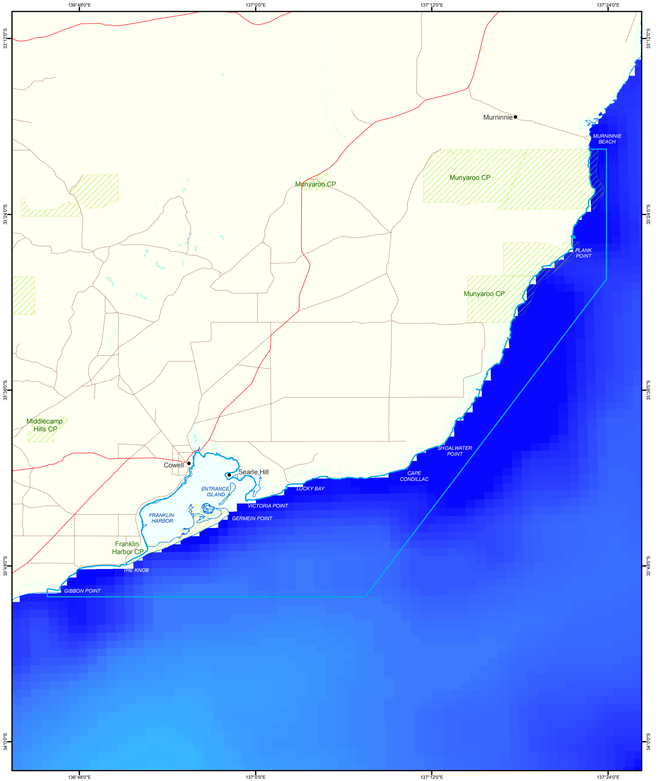
Figure 11: Franklin Harbor Marine Park Average Winter Sea Surface Temperature
