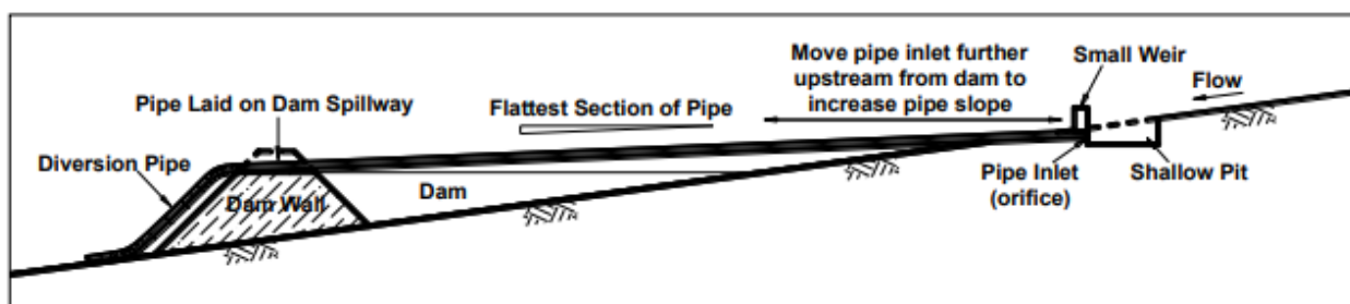
Figure 7: Profile of Device showing Pipe Slopes
