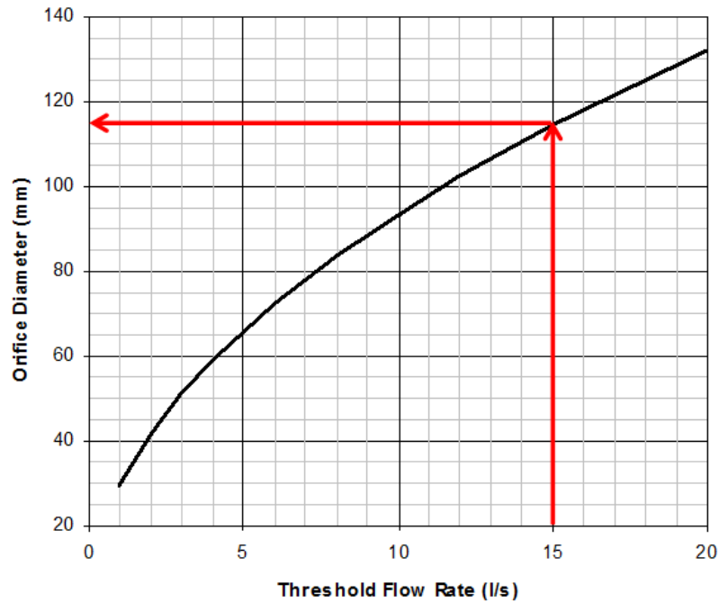
Figure 5: Orifice Diameter versus Threshold Flow Rate (1 – 20 l/s)
