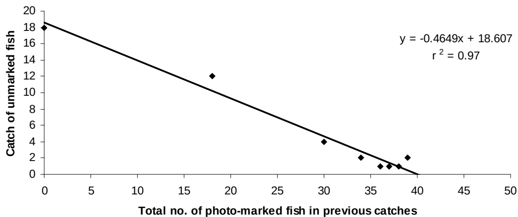
Figure 18. Estimate of total population size at Seacliff Reef using the pseudo-removal method. The intersection of the fitted regression line with the x-axis gives a total population estimate of N = 40 fish.
