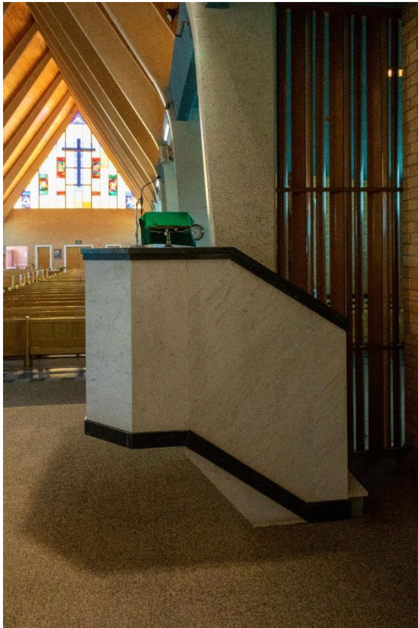
Cantilevered pulpit
