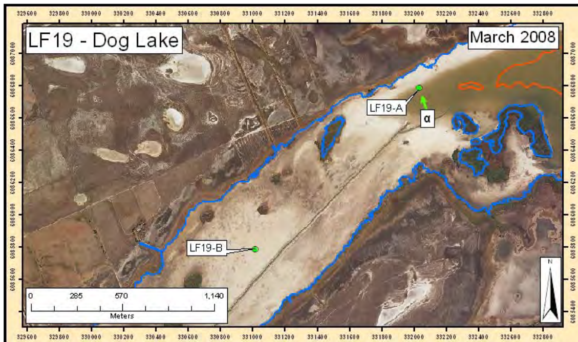
Figure 16-1 Sample location map. Aerial photograph taken in March 2008 (Orange line: sampling-b water level, Blue line: sampling-c, d, e & f water level)
