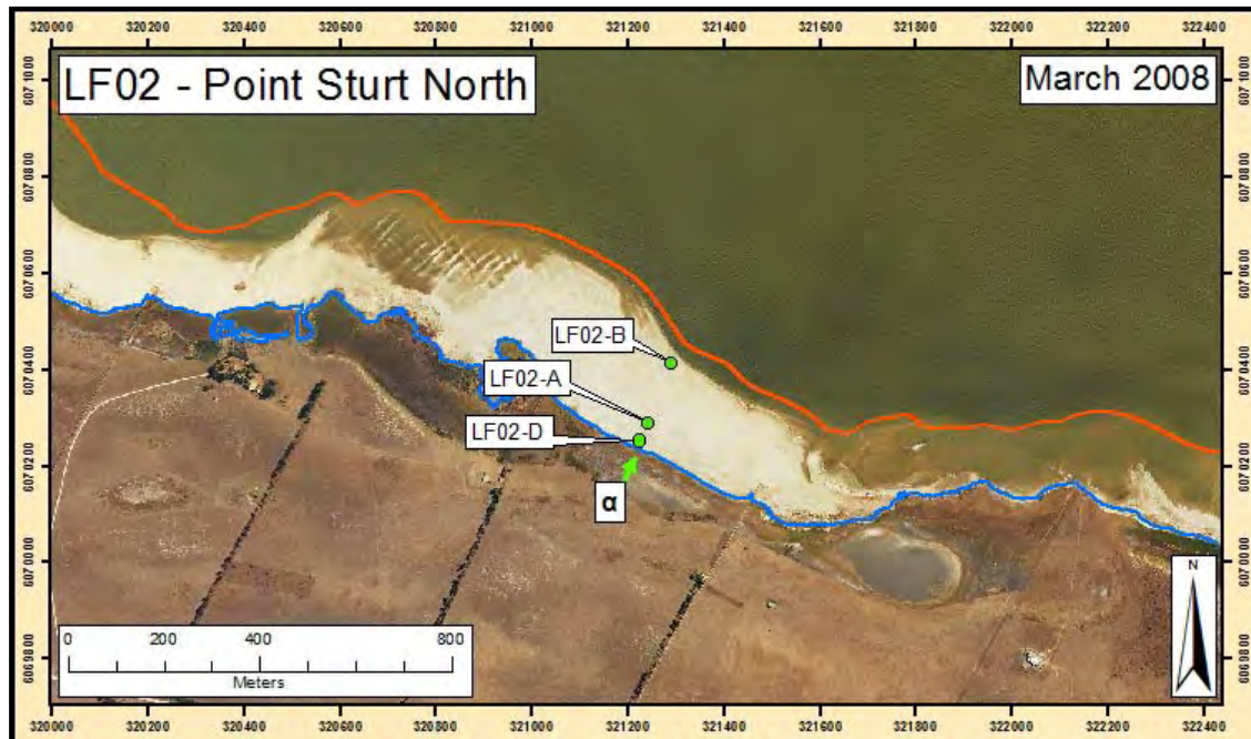
Figure 5-1 Sample location map. Aerial photograph taken in March 2008 (Orange line: sampling-a & b water level, Blue line: sampling-c, d, e & f water level)
