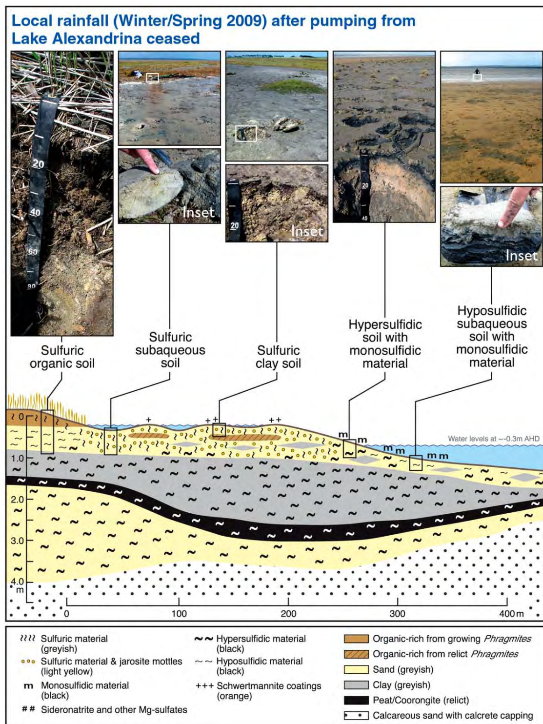
Figure 22-4 Descriptive toposquence model for an area near Campbell Park in Lake Albert showing spatial variation of ASS materials after several winter rainfall events (winter / spring 2009)
