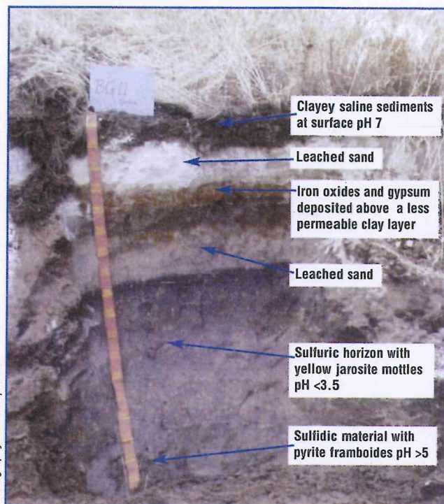
Figure 1a Actual acid sulfate soils showing yellow streaks and mottling patterns containing jarosite (pH < 4) in the grey subsoil
