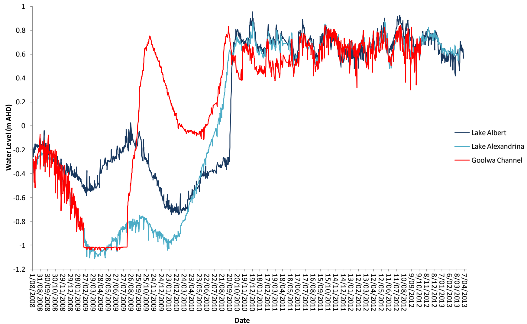
Figure 2: Daily mean water levels in Goolwa Channel (Signal Point), Lake Alexandrina (Milang) and Lake Albert (Meningie) from August 2008 to April 2013 (except Goolwa Channel August 2008 to November 2012) (Department for Environment, Water and Natural Resources 2013b).
