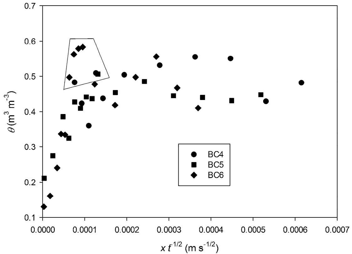
Figure 18. Water content ( \theta ) versus Boltzman transform ( xt^{1/2} ) for Boggy Creek cores. The data enclosed in the box were removed from the data set as being unreliable when fitting eqn (7).
