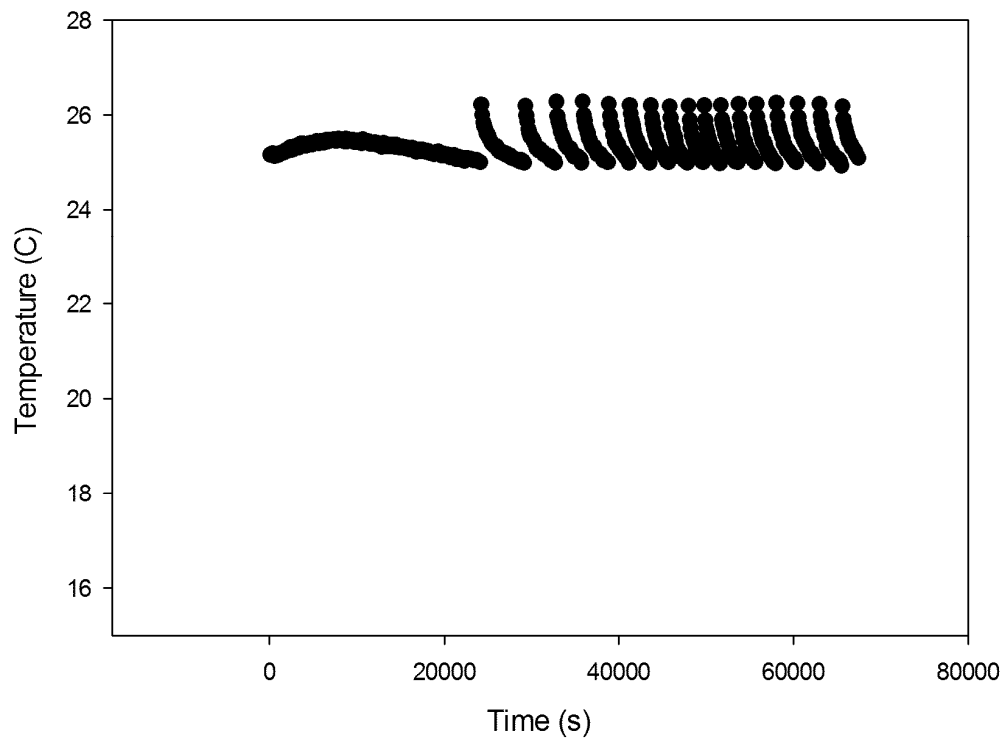
Figure 12. Temperature versus time for box. The initial period before the switching can be seen is due to the box temperature being > 25^{\circ}\text{C} .
