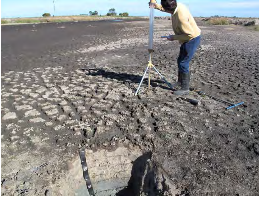
Figure 25. Photograph showing cracking of sediments and infilling at Boggy Creek site. (Photograph by Dr R. W. Fitzpatrick).
