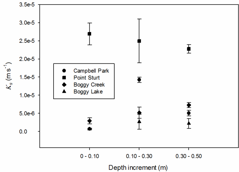
Figure 27. Saturated hydraulic conductivity ( K_s ) range and mean for the four sites derived from the particle size data using the method of Saxton et al. (1986).
