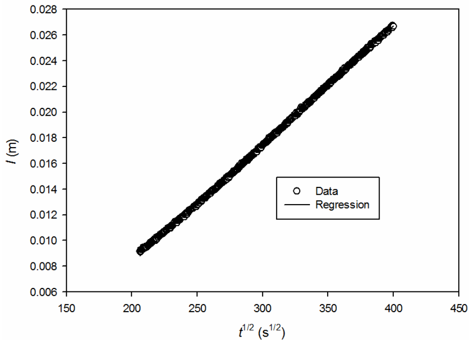
Figure 17. Evaporation (m) versus square root of time ( \text{s}^{1/2} ) for core PS5 during the second stage of drying.
