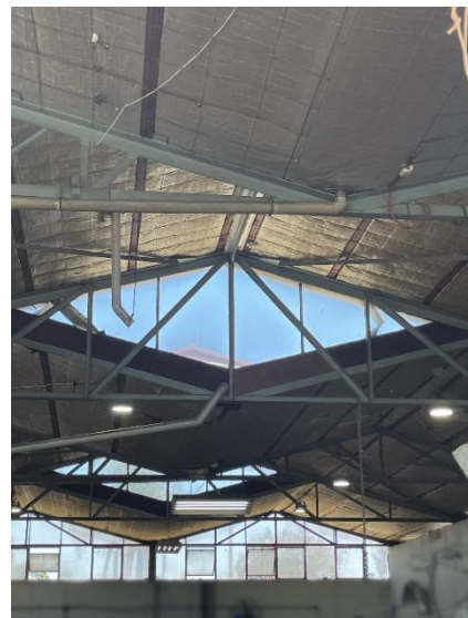
Roof trusses in factory forming rhomboid skylights.
